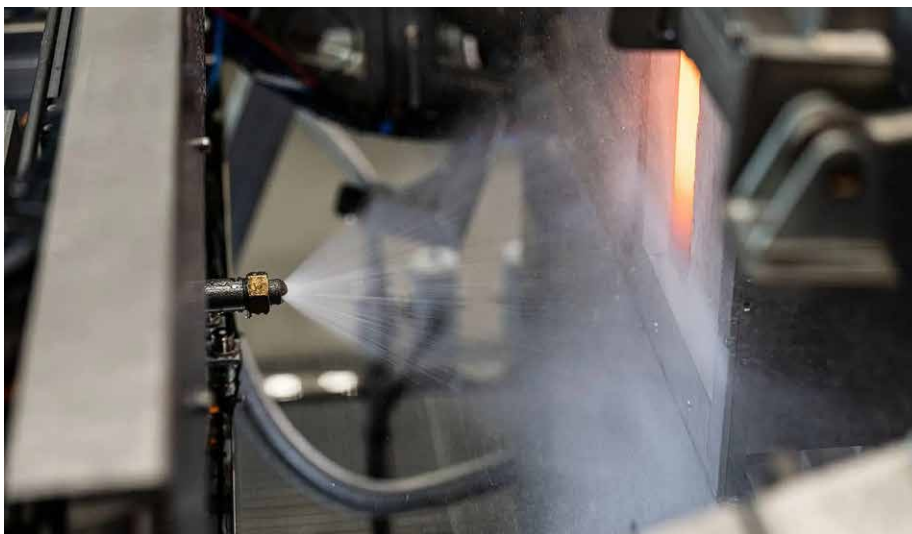
The measuring plate is equipped with a temperature probe, and the equipment can fully rotate (Picture: Primetals Technologies)
