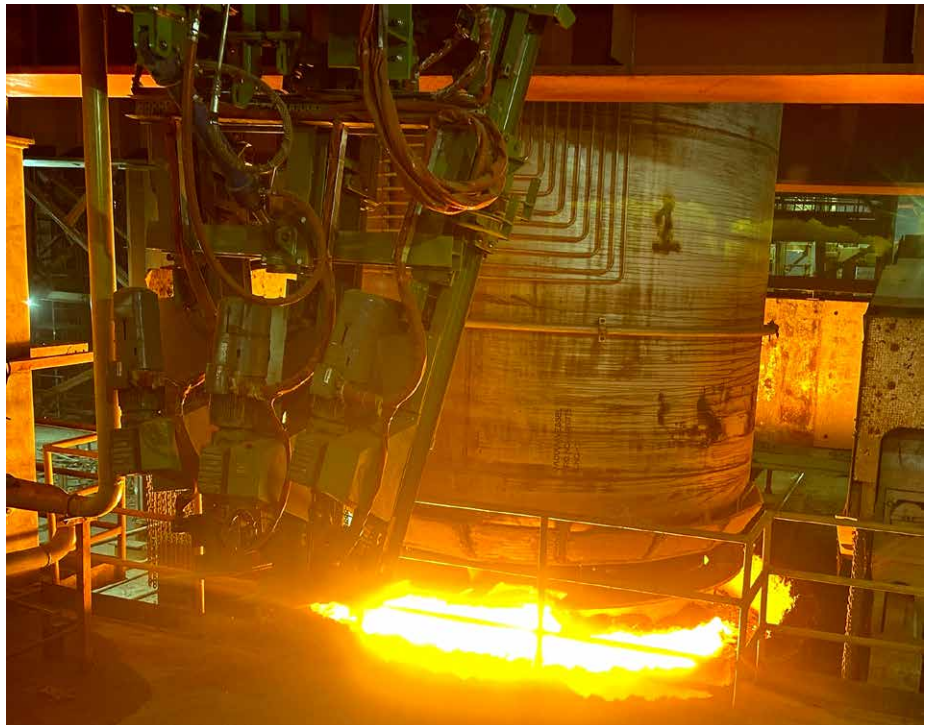
First heat of the 350-ton RH plant at JSW Vijayanagar works steel plant 4 in Toranagallu, India (Picture: SMS group)
