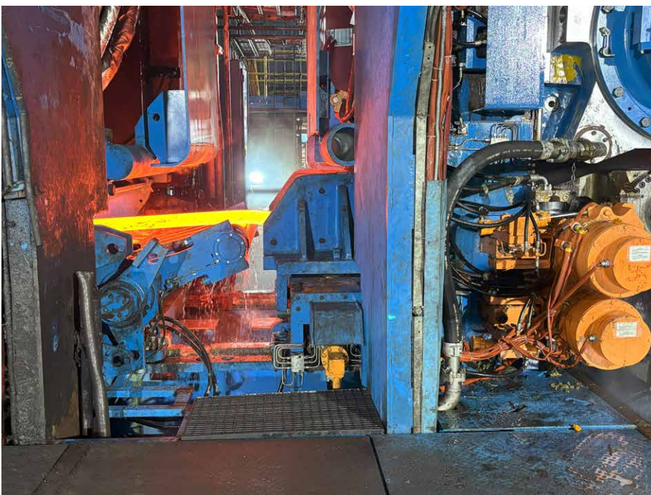
The upgraded Tata Steel TSCR plant can now roll high-quality coils down to one millimetre thickness (Picture: SMS group)
